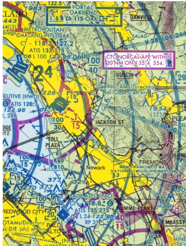
Figure 9.9: Oakland VOR and 114 radial to MISON intersection
