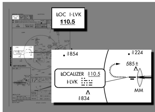
Figure 9.17: Livermore 25R localizer
