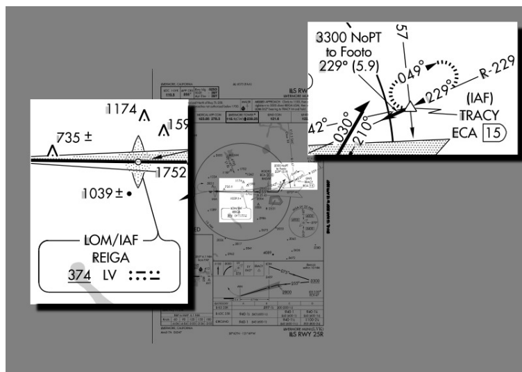
Figure 9.12: Initial approach fixes
